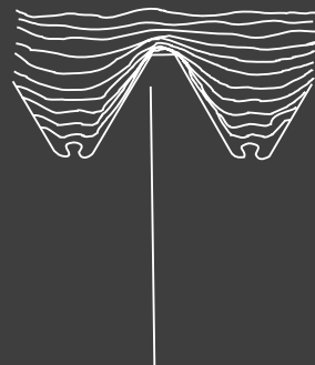
Fibre structure of thread forming 挤压丝锥攻丝后的组 织结构
