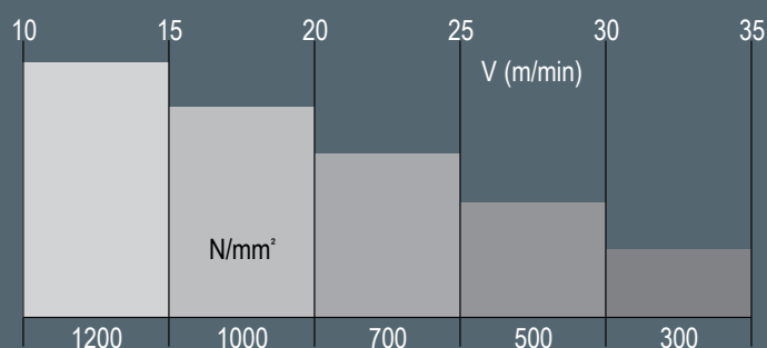
Material toughness
